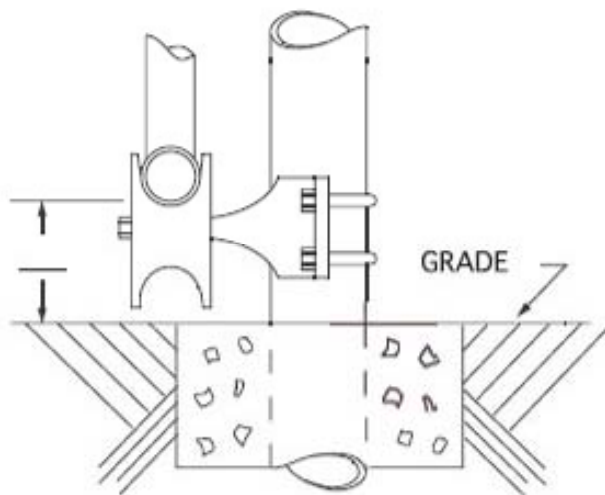
1 ROLLER DETAIL
