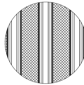
PALE W/ \frac{3}{16} " RND X \frac{1}{2} " 18GA PERF
